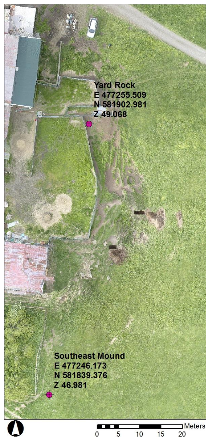
Figure 23. GNSS measured base points for total station set up.
