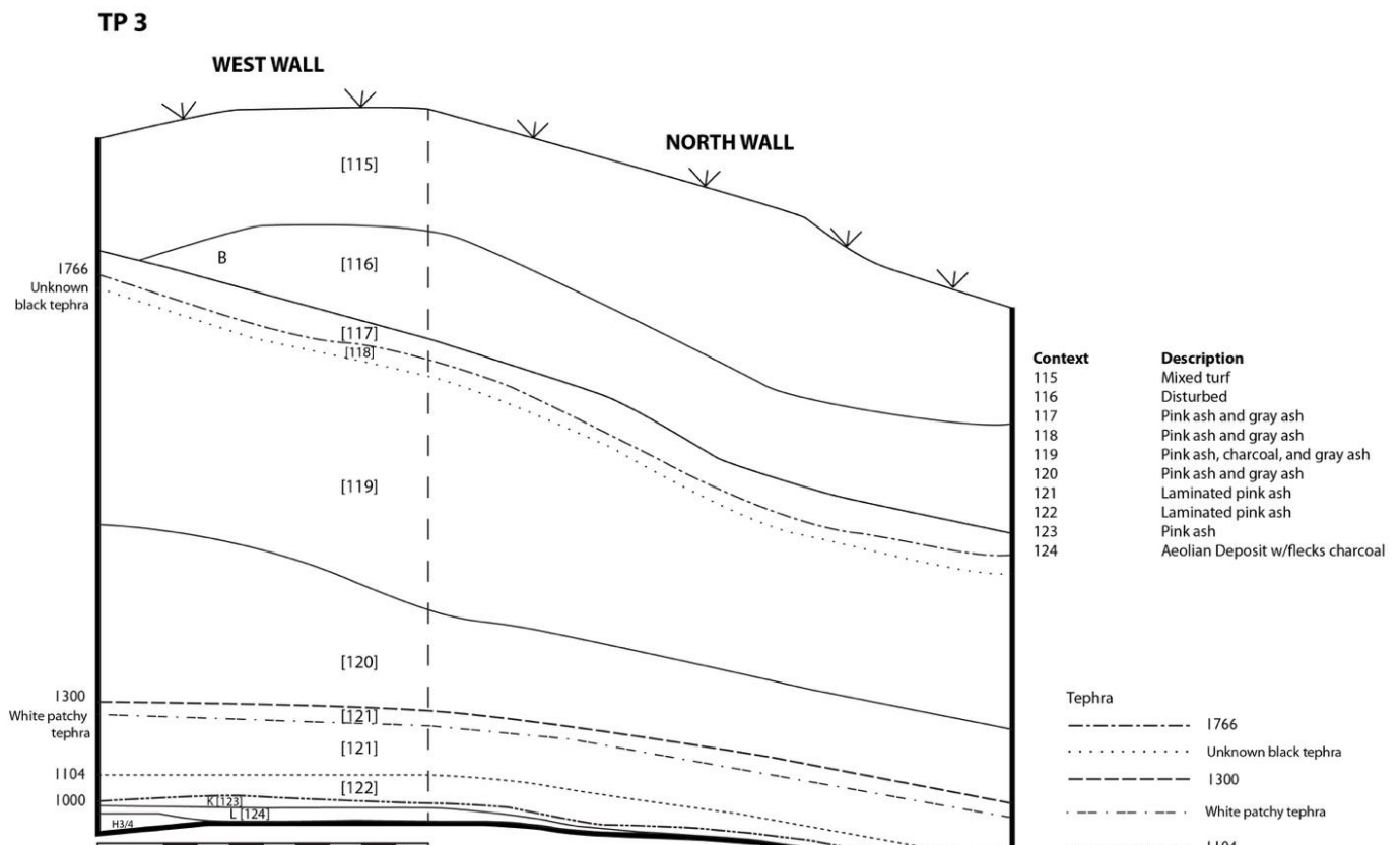
Figure 4. Test pit 3 profile.
